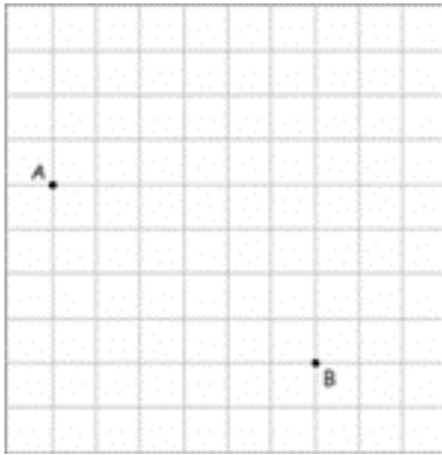
Figure 6-2. Grid-world task.
